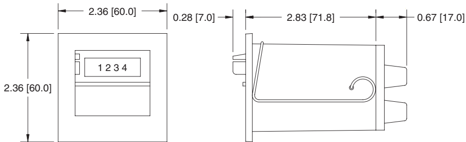
Panel cutout: 2.17" x 2.17" [55.1 x 55.1]
